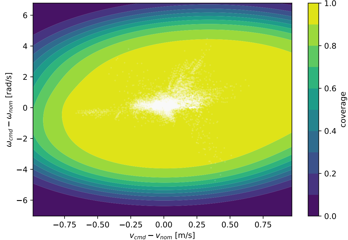
Residual coverage vs command offset (0 = off / OOD; state fixed at mean [0.57 m/s, 0.20 rad/s])
